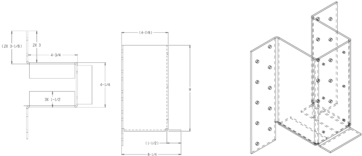
FIGURE 1 – MTWDeck Bracket
