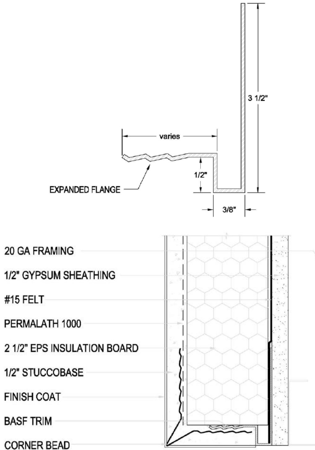
Figure 1 – Typical opening detail for NFA 285 assembly (See Table 5)
