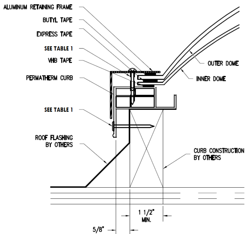
Figure 3 – DDCS, ECS, and DDRCS Curb Attachment Detail
