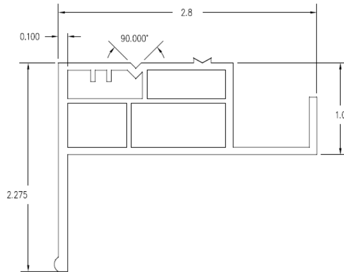
Figure 4 –Permatherm Curb Cross-section Profile
